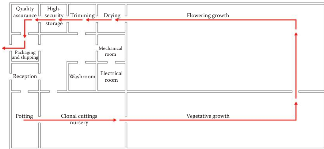
FIGURE 14.2 Simplified layout of a professional marijuana production facility. The red arrows indicate the sequence of production and processing. Designed by Steve Naraine.
