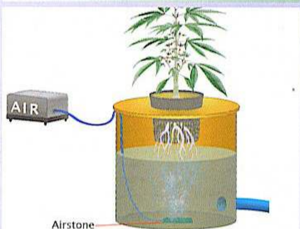
Cutaway of the inside of a DWC garden
