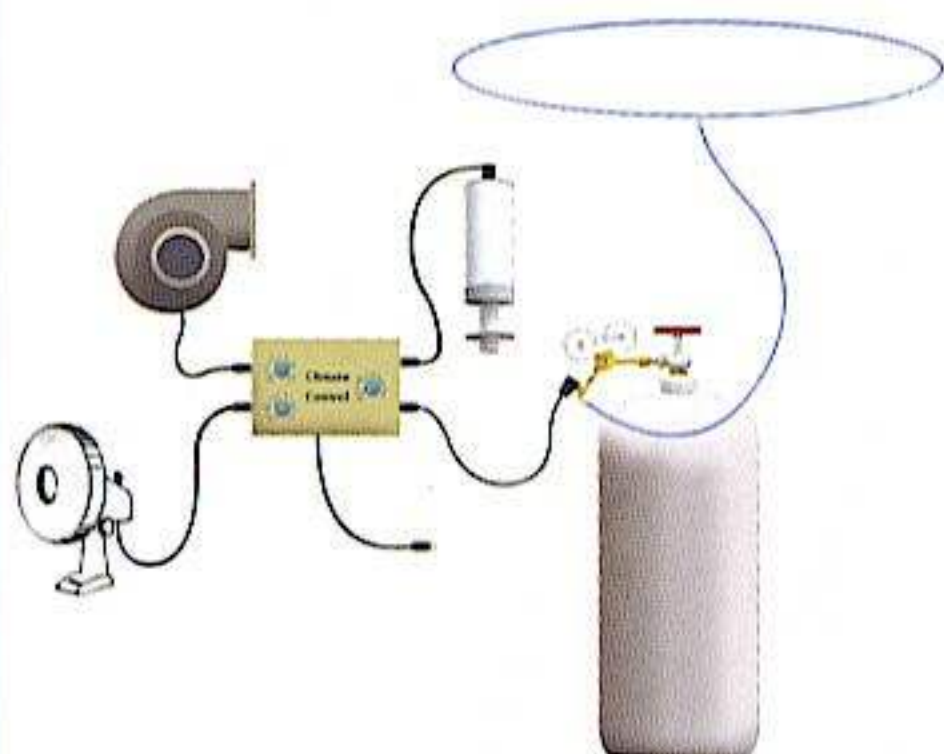
A set-up consists of a tank of CO 2 gas, regulator, solenoid valve, and a flow meter.
