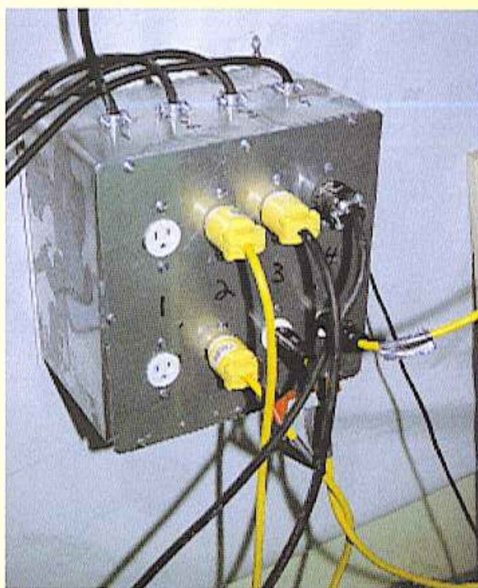
BC growers run flowering rooms 24 hours a day with half as many ballasts. This box is made for three transformers, capacitors, and starters to run six 1000-watt HP sodiums. Three lamps run for 12 hours; the other three lamps run for the next 12 hours.
