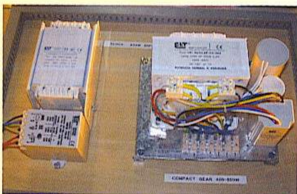
Ballast designs are more simple now than ever before. Above, you see two new European ballast designs.
