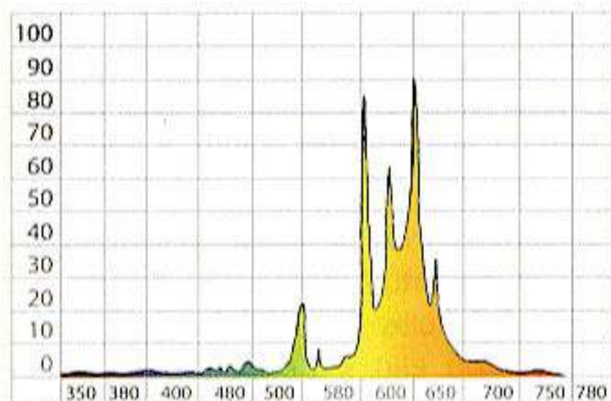
Color spectrum of Son Agro bulb
