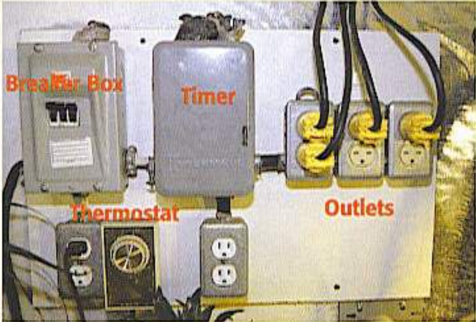
Wiring your own grow room is relatively easy. This grower hardwired a separate breaker box and timer that supports four lamps.
