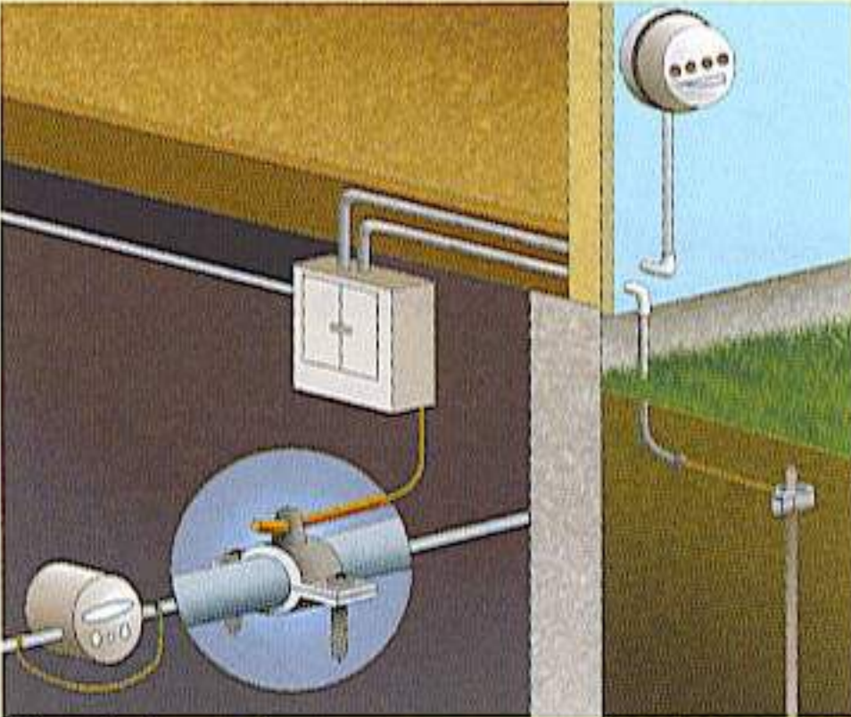
Electrical ground
